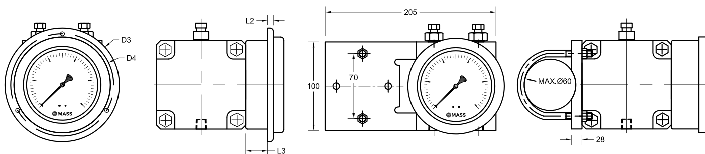
Front Panel Mounting
